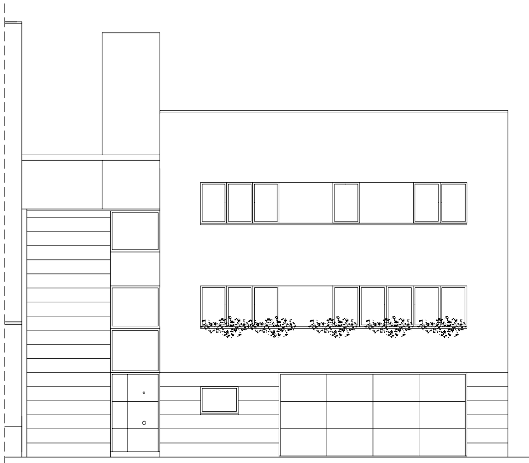
Façana Principal
